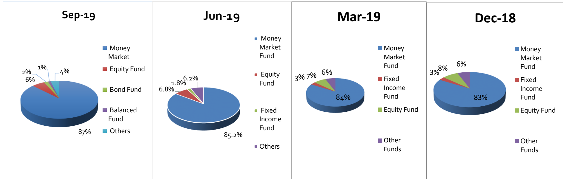
Figure 4: Percentage of investments per category of fund
